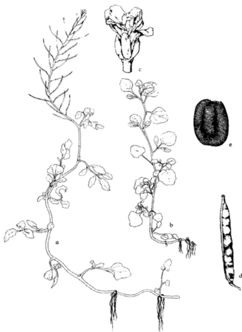
Fig. 129. Nasturtium microphyllum : a. habit, flowering and fruiting; b. habit, vegetative; c. flower; d. fr. c. seed (CS&W). Crow and Hellquist, 2000
